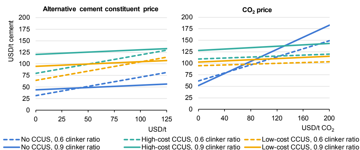
Figure 4.19 Levelised cost of cement production under varying techno-economic assumptions
